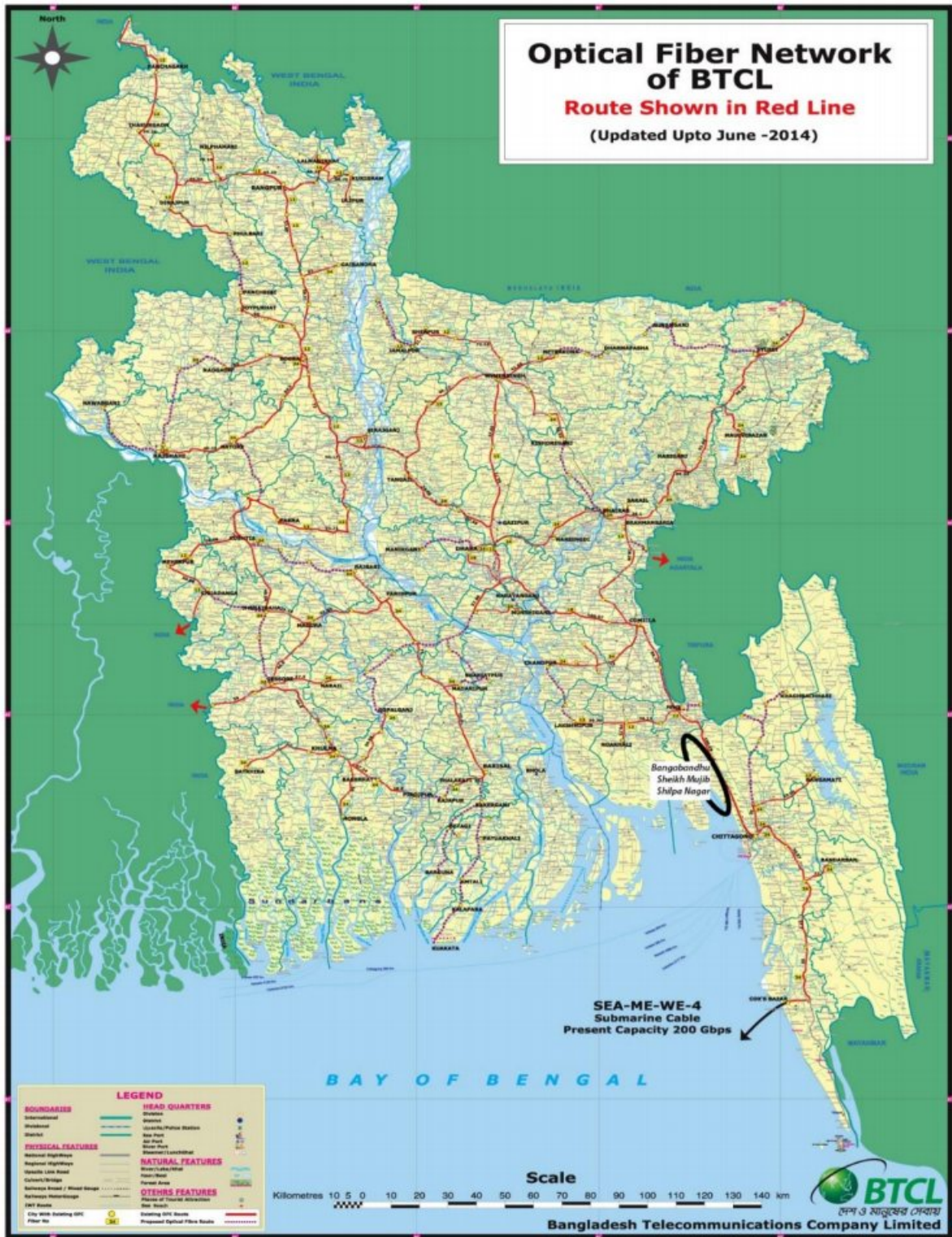
Figure 4-26: Optical Fiber Network of BTCL
